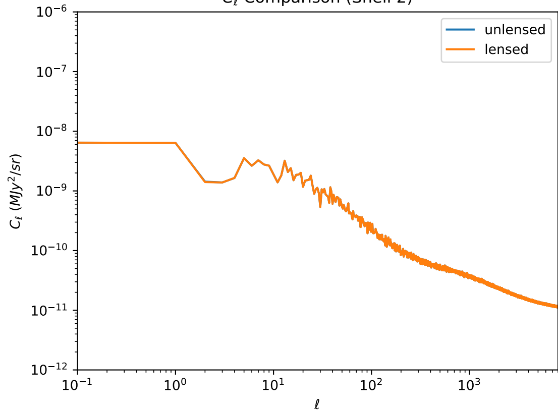
C_\ell Comparison (Shell 2)
